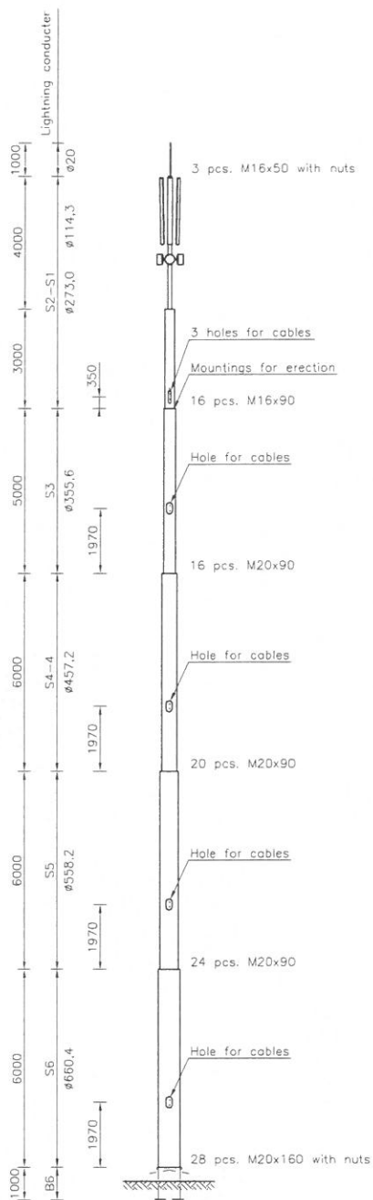
30m Monopole, 1:100
